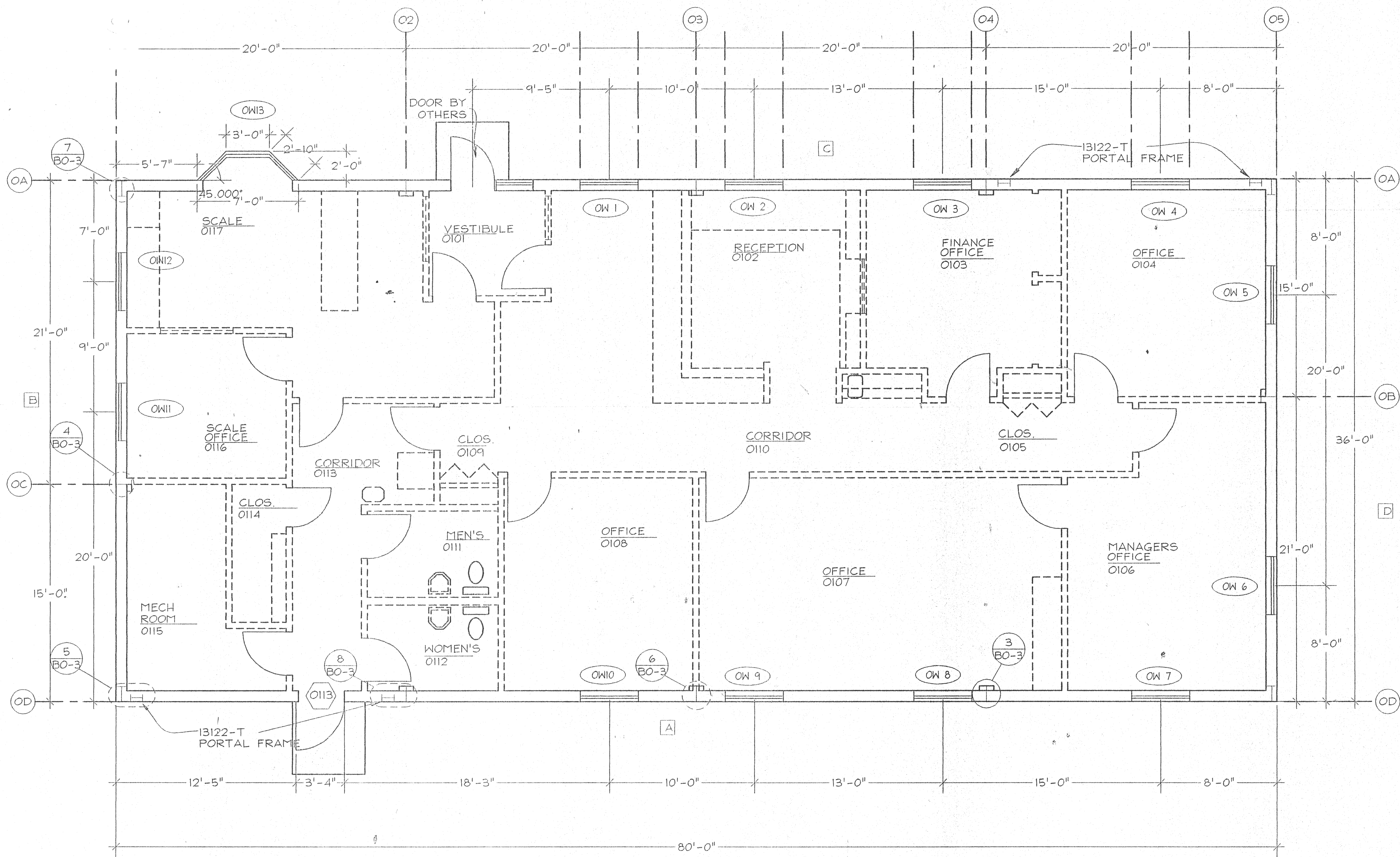
1 OFFICE FLOOR PLAN SCALE: 1/4"=1'-0" NORTH
