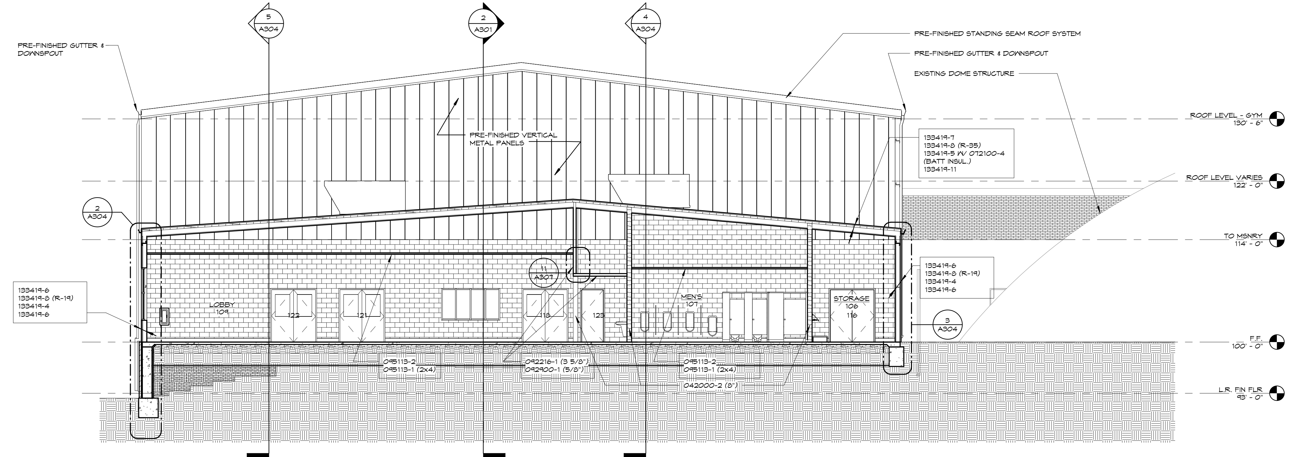
1 E-W SECTION THROUGH LOBBY AND RESTROOMS LOOKING SOUTH 1/8" = 1'-0"
