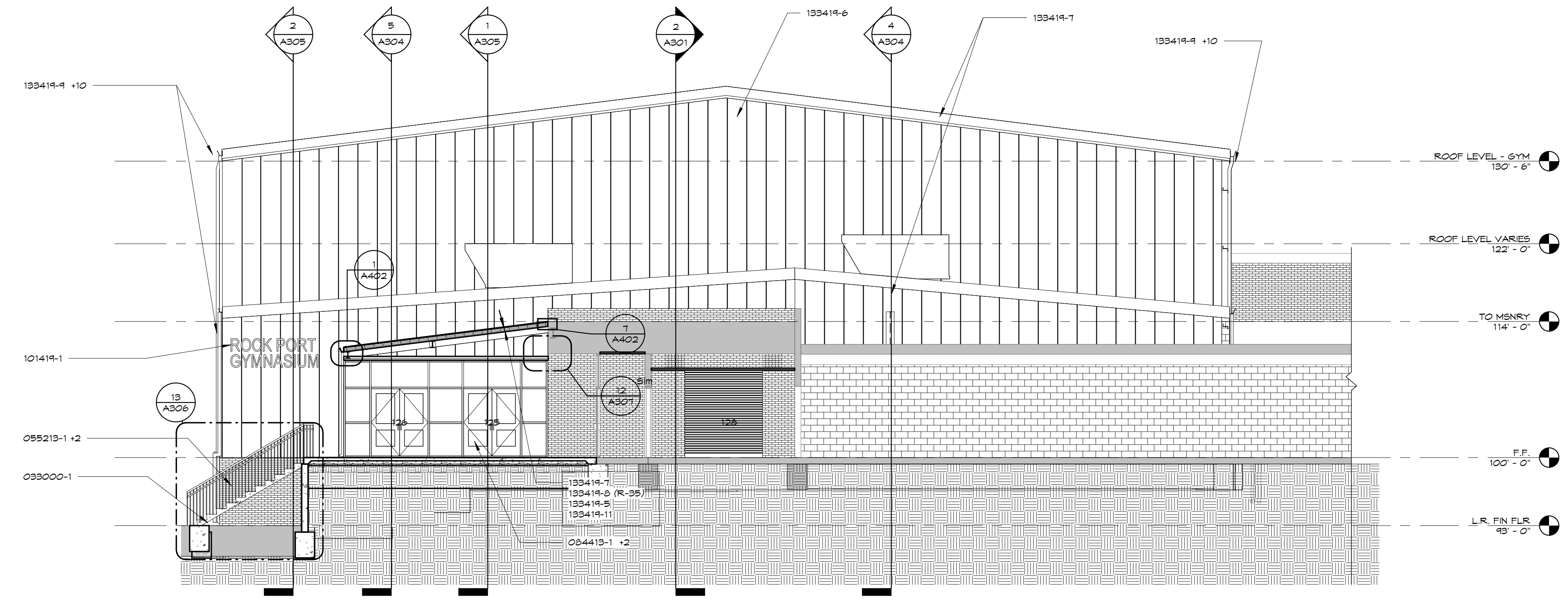
2 E-W SECTION THROUGH ENTRY LOOKING SOUTH 1/8" = 1'-0"
