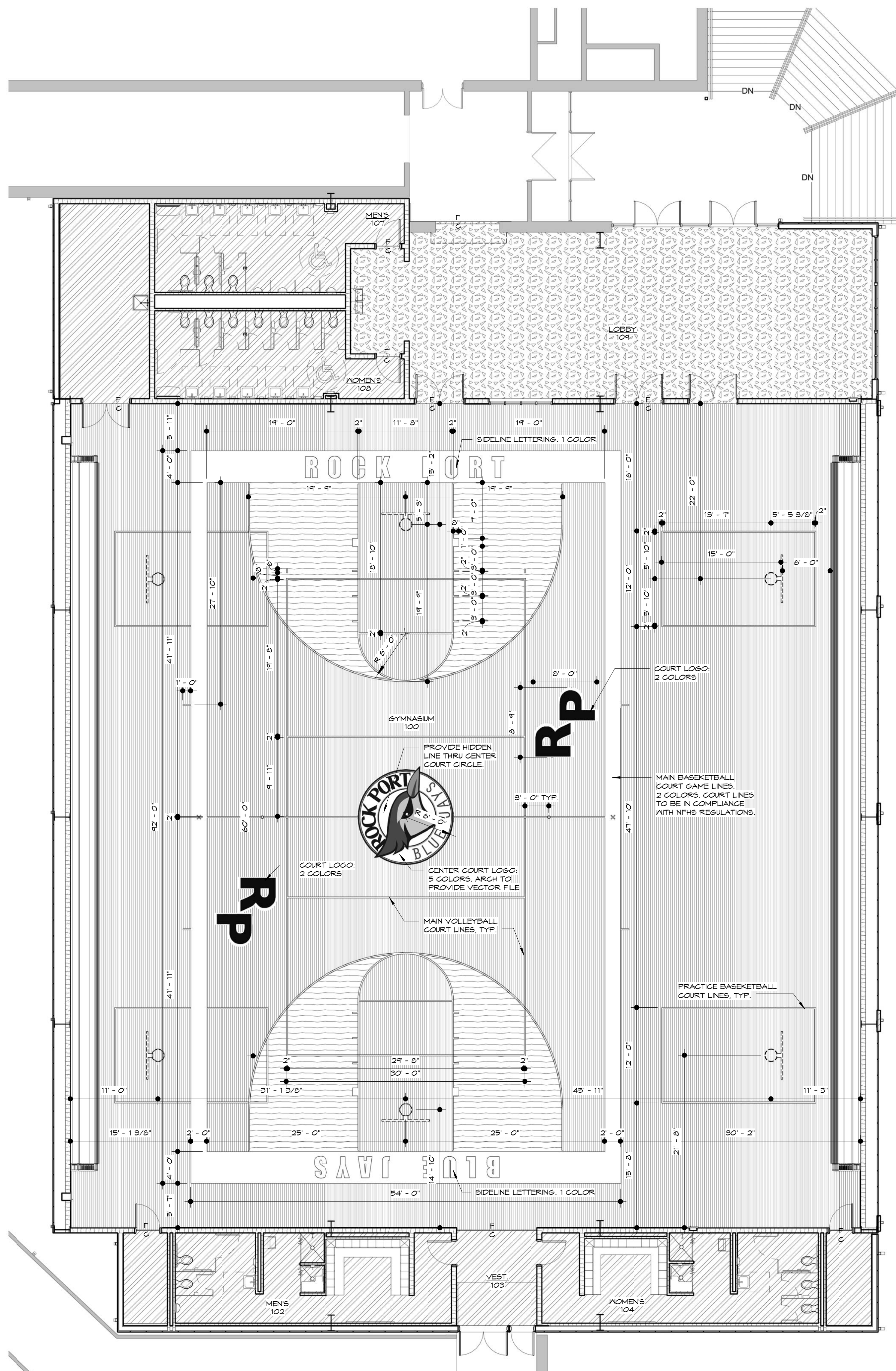
1 FINISH FLOOR PLAN 1/8" = 1'-0"
