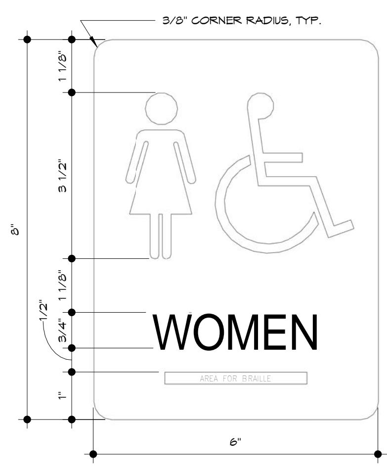
6 SIGN TYPE A 6" x 1'-0"
