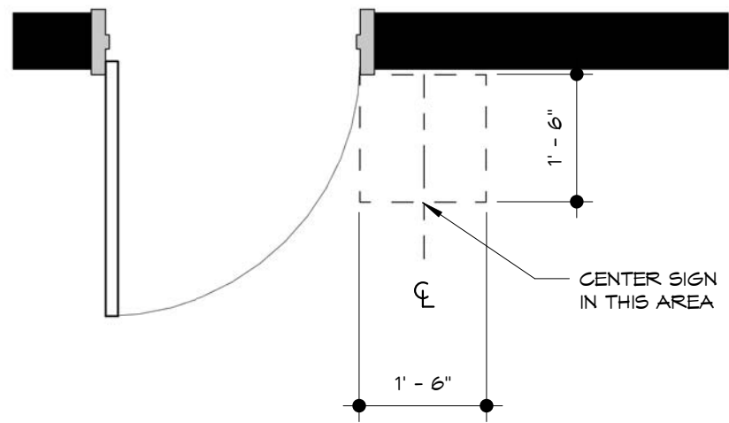
SIGN LOCATION DETAIL
