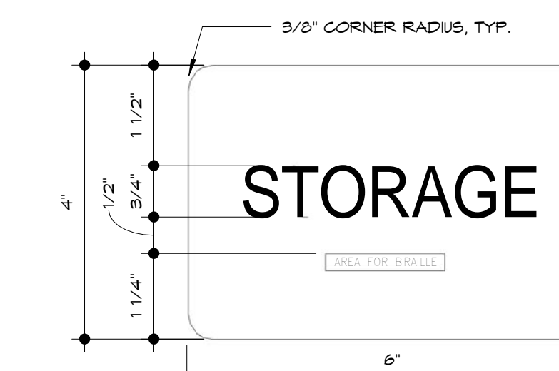
7 SIGN TYPE E 6" x 1'-0"
