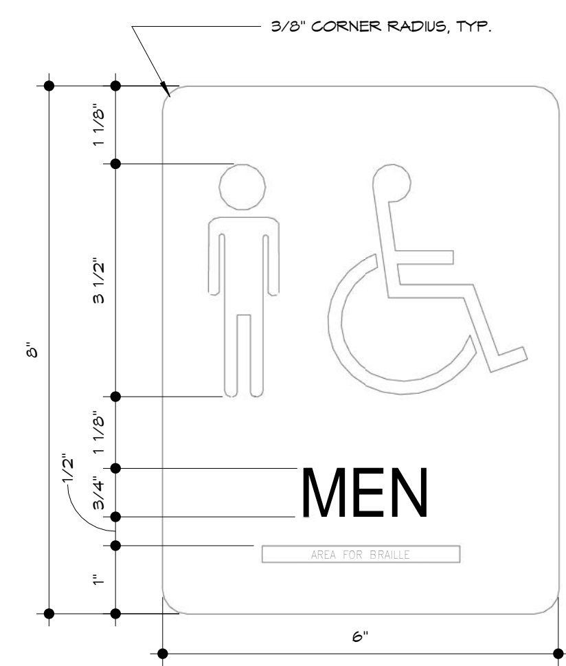
5 SIGN TYPE B 6" x 1'-0"
