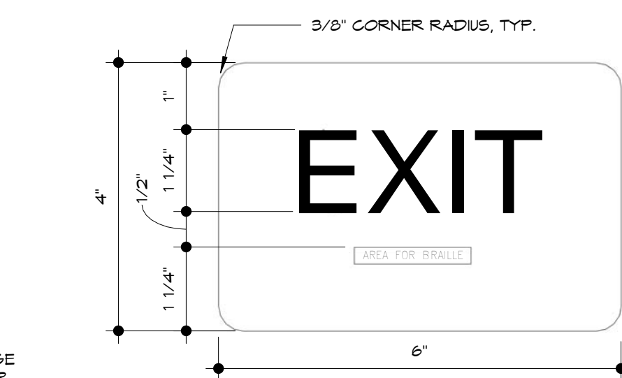
2 SIGN TYPE D 6" x 1'-0"
